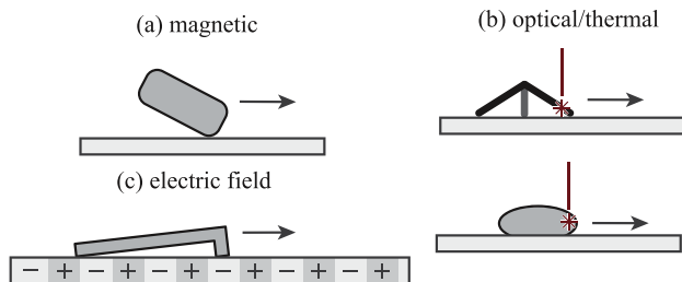
Fig. 2. Some existing off-board approaches to mobile microrobot actuation and control in 2D. (a) Magnetically driven crawling robots include the Mag- \mu Bot [33], the Mag-Mite magnetic crawling microrobot [59], the magnetic microtransporter [60], rolling magnetic microrobot [61], the diamagnetically-levitating mm-scale robot [62], the self-assembled surface swimmer [63], and the magnetic thin-film microrobot [64]. (b) Thermally driven microrobots include the laser-activated crawling microrobot [31], microlight sailboat [43], and the optically controlled bubble microrobot [39]. (c) Electrically driven microrobots include the electrostatic scratch-drive microrobot [65] and the electrostatic microbiorobot [60]. Other microrobots which operate in 2D include the piezoelectric-magnetic microrobot MagPieR [66] and the electrowetting droplet microrobot [67].
